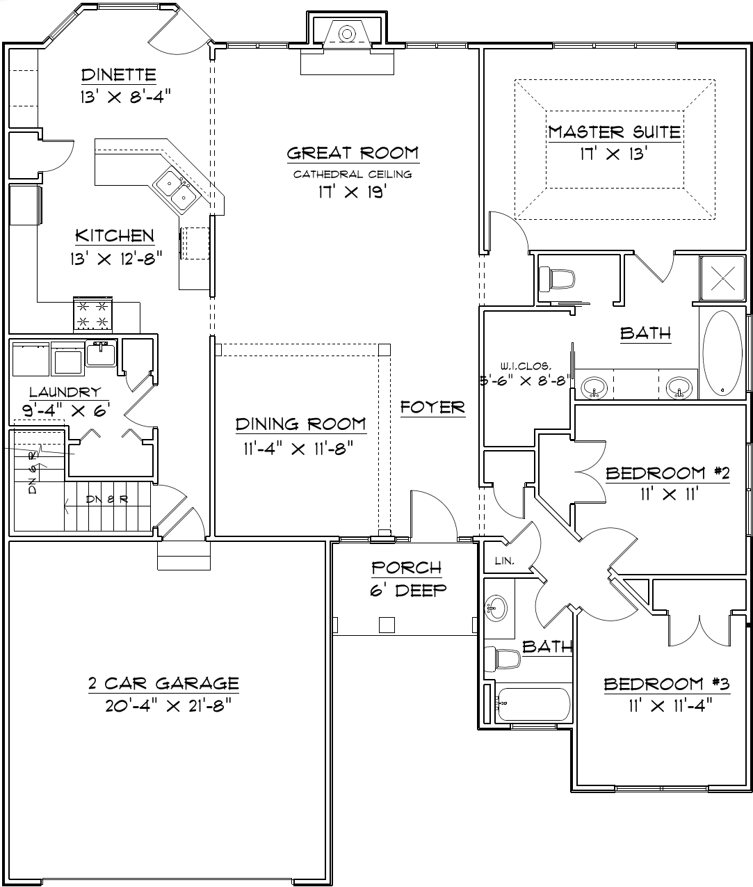
MAIN FLOOR PLAN SCALE: 1/4" = 1'-0"
