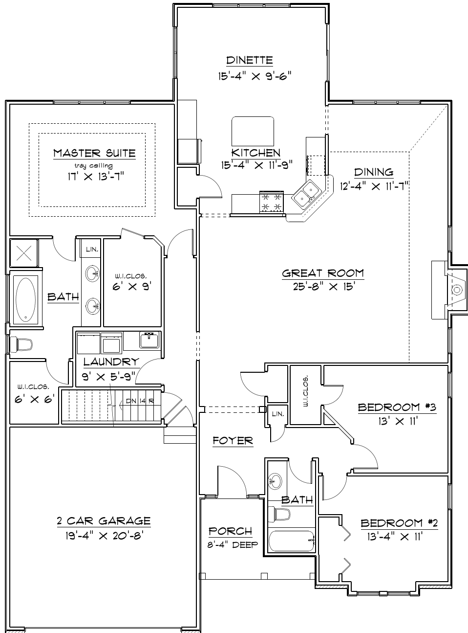
MAIN FLOOR PLAN SCALE: 1/4" = 1'-0"
