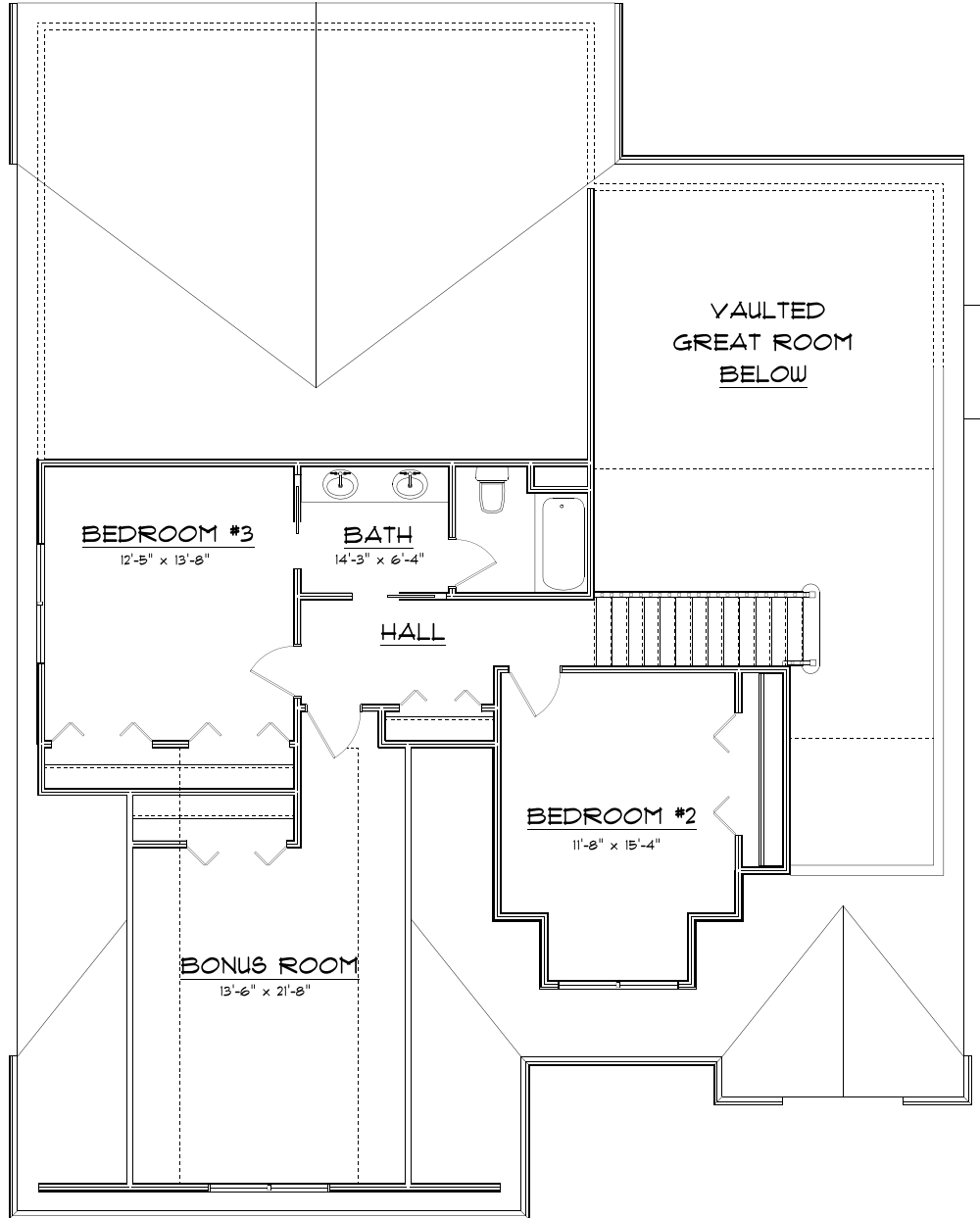
SECOND FLOOR PLAN 609 SQ. FT. + 297 BONUS ROOM
