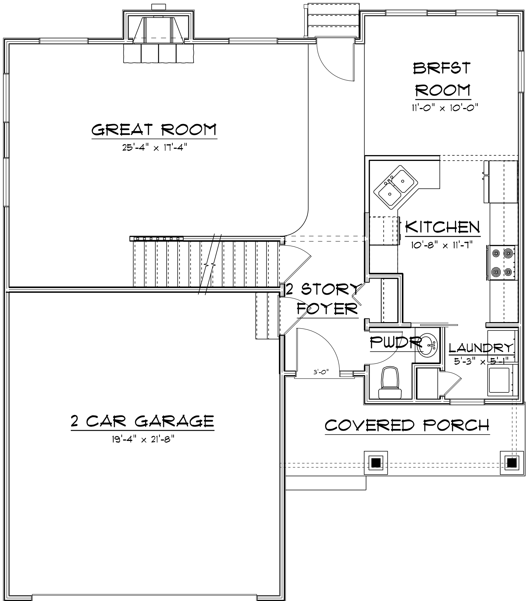
FIRST FLOOR PLAN 816 SQ. FT.
